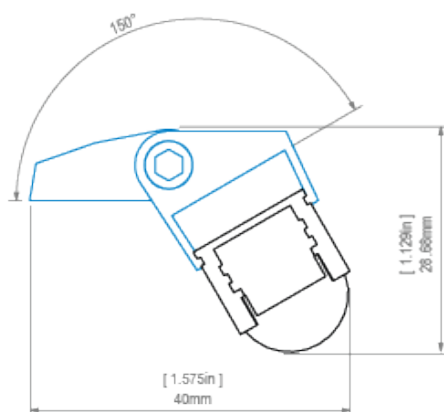
REGULOR extrusion and REG-PD-UV mounting bracket
