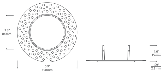
*SHIPS WITH MUD/PLASTER PLATE FOR FLANGELESS INSTALLATION
